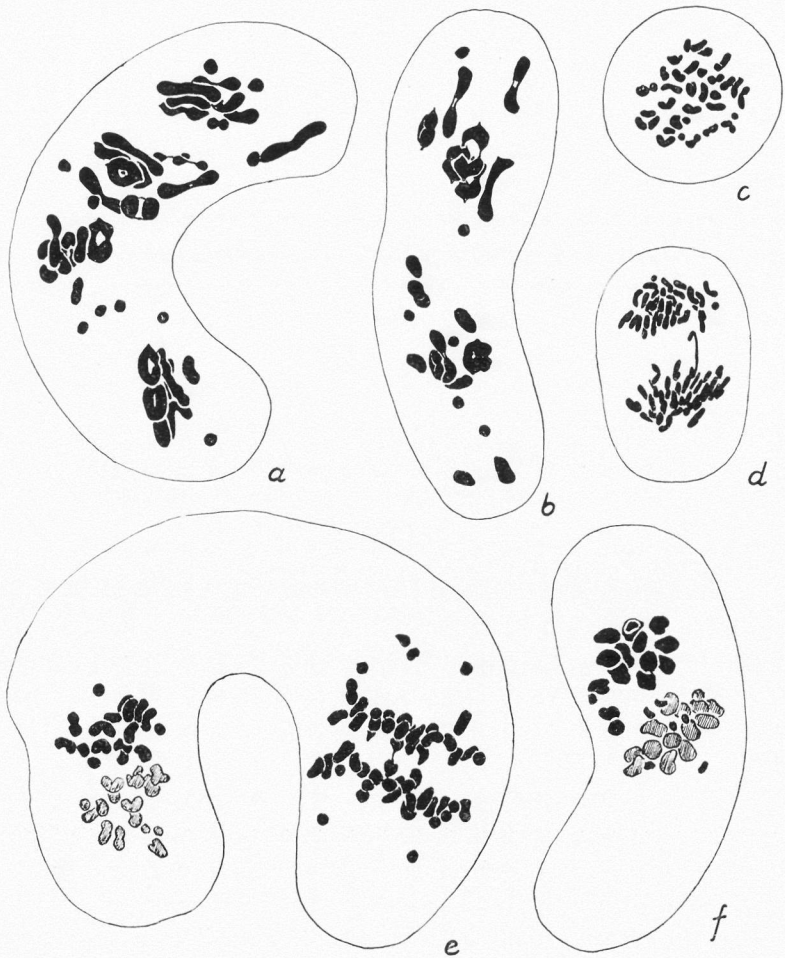
Fig. 7. Syncyte formation in Phleum phleoides no. 462. — a—b examples of syncytes in which the individual fused PMCs spindles have been preserved apart (see text). — c—d syncytes in anaphase II (polar and side view) with about 28 A-chromosomes on the same spindle. — e—f syncytes in anaphase I, in e there is on the right a spindle with 21 separating A-bivalents and on the left a spindle with about 14, in f there are four B-chromosomes already divided and 14 separated A-bivalents. \times 2200 .
