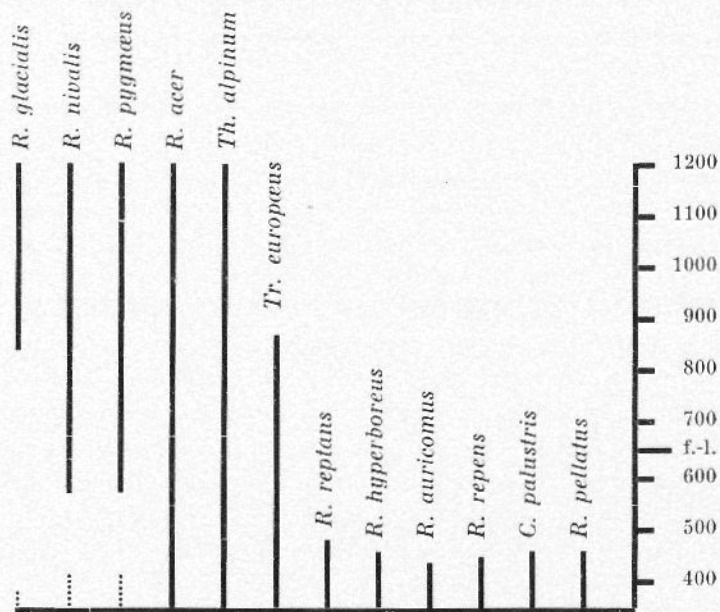
Fig. 1. The vertical distribution of Ranunculaceae on Nuolja. — f.-l. = forest-limit.
