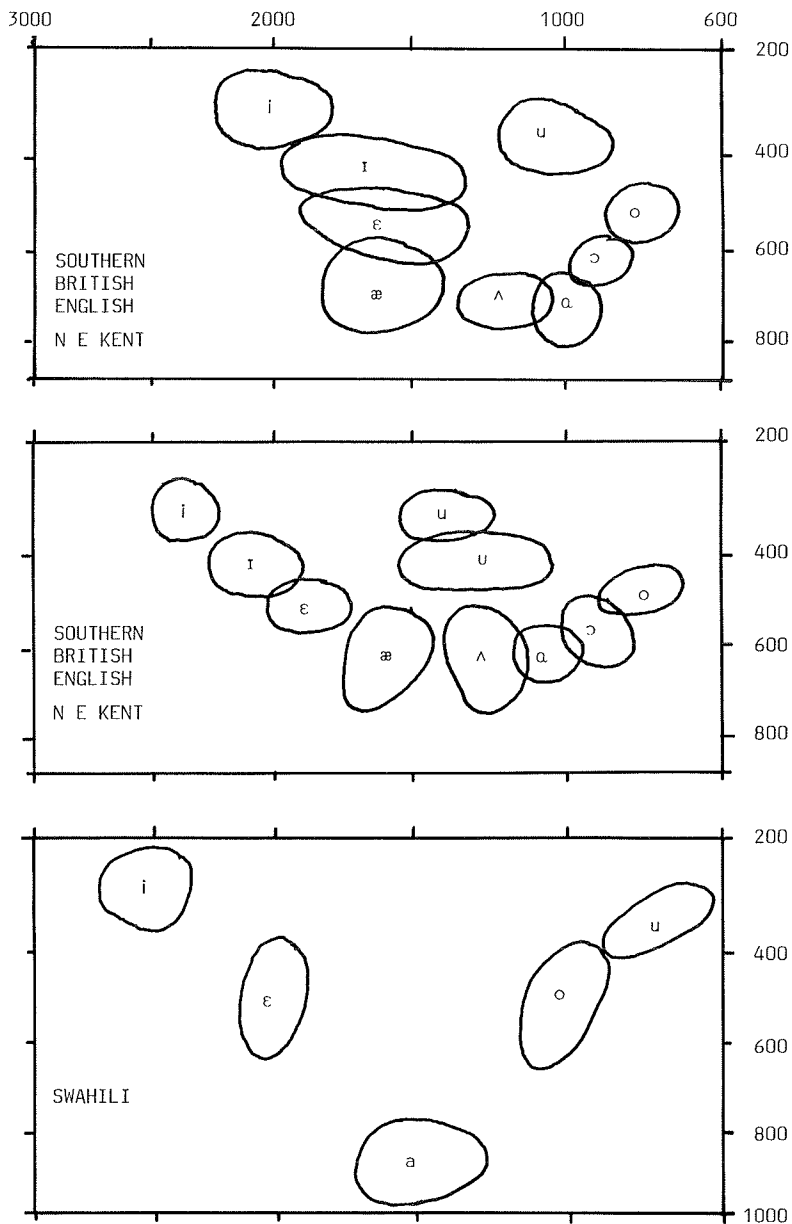
Fig. 11 Frequencies of F1 and F2 from stressed vowels in continuous speech by three adult males.
