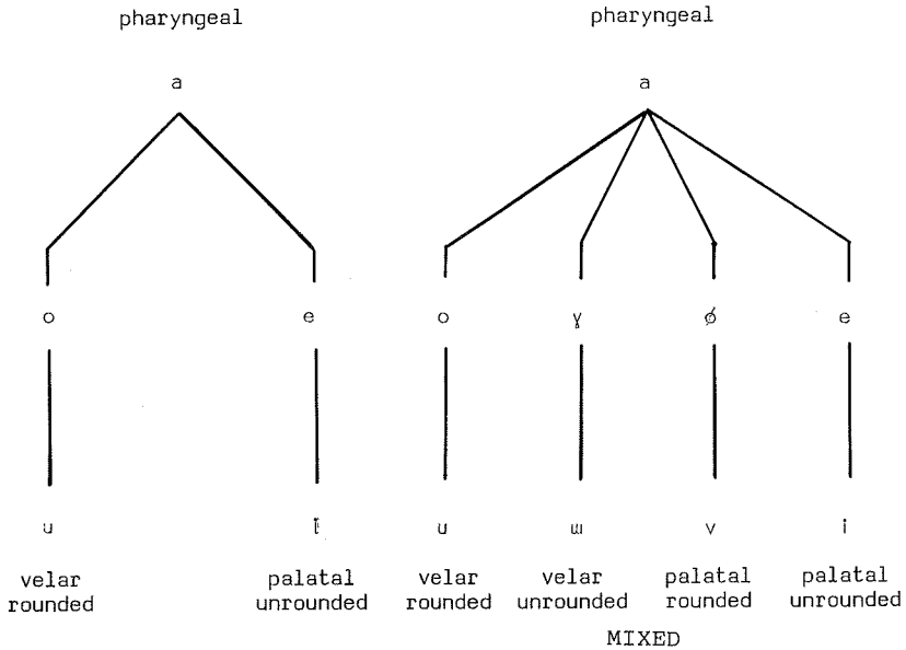
Fig. 2 In the early years of the 19th century the ancient model was commonly portrayed as trees with palatal and velar series branching off from a basic pharyngeal configuration. Vowels in each branch are differentiated by open vs close jaw position. The mixed branches combine the spread lips of the palatals with the velar tongue manoeuvre and the rounded lips of the velars with the palatal tongue manoeuvre.
