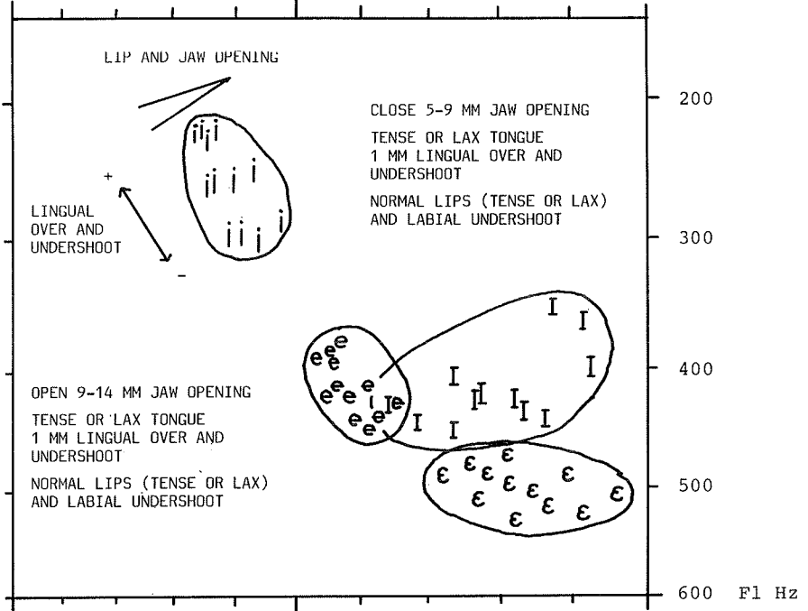
Fig. 17 Variation of F 1 and F 2 generated by varying the jaw position and allowing \pm 1 mm of lingual precision and \pm 2 mm of labial position for different combinations of tense and lax tongue postures and open and close jaw positions, as illustrated in Fig. 16.
